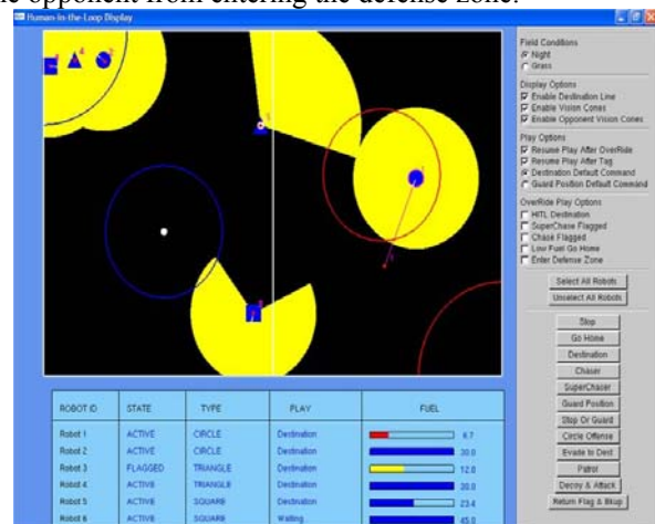
Figure 1. RoboFlag 2.0 interface.
